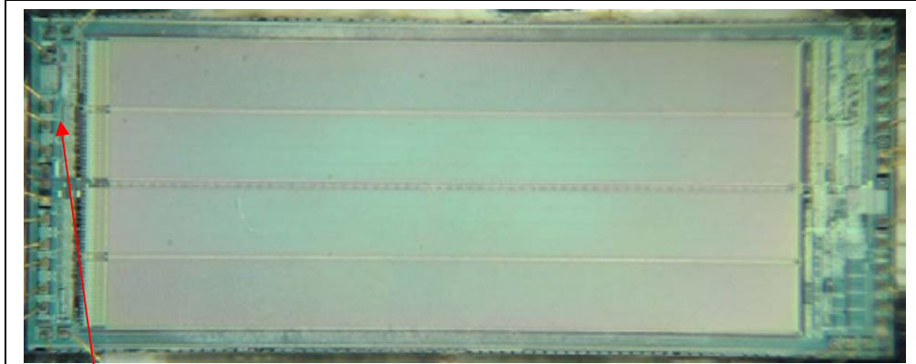
Figure3. Device Die (MAG 35X)
